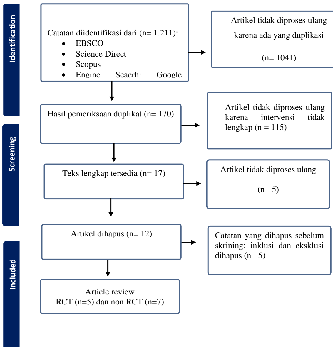
Gambar 1. Prisma Flow Chart
